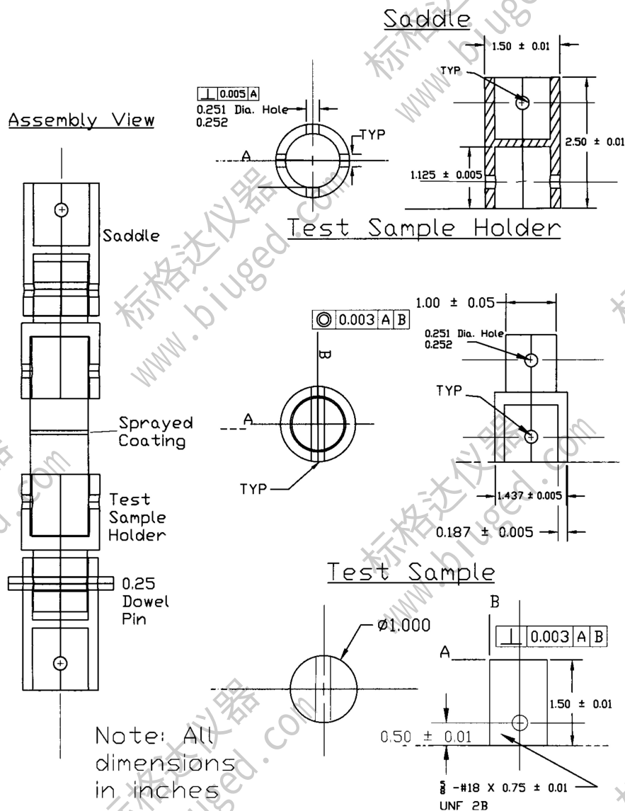
FIG. X1.1 Alternative Load Train Geometry for Test Assembly
