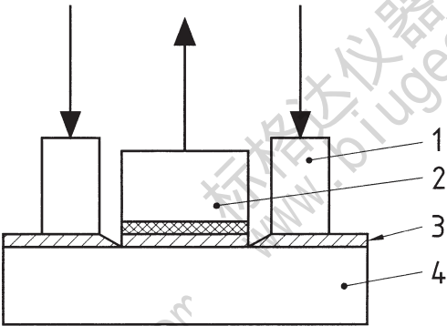
Figure 5 — Test assembly for rigid substrates
