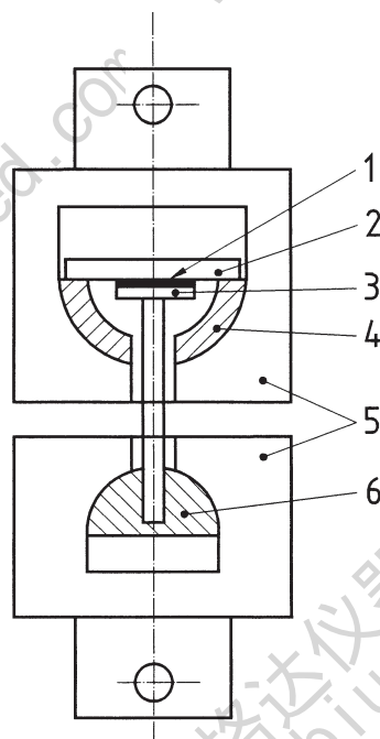
Figure 2 — Example of a suitable test apparatus for the method described in 9.4.2
