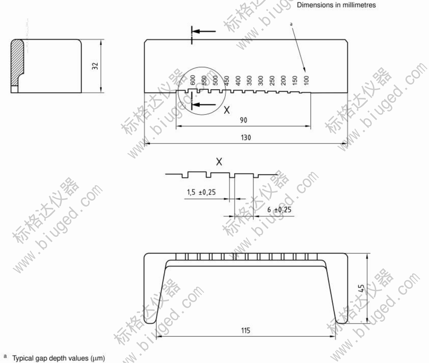
Figure A.2 — Typical sag index applicator blade (type 2)
