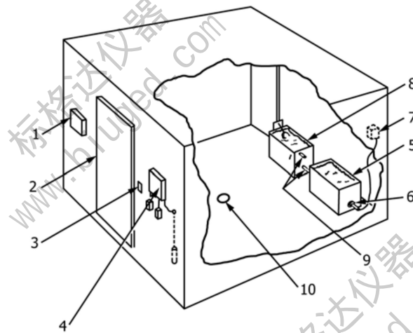
FIG. X1.1 Humidity Cabinet
