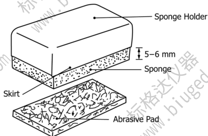
FIG. 2 Abrasion Boat Components
