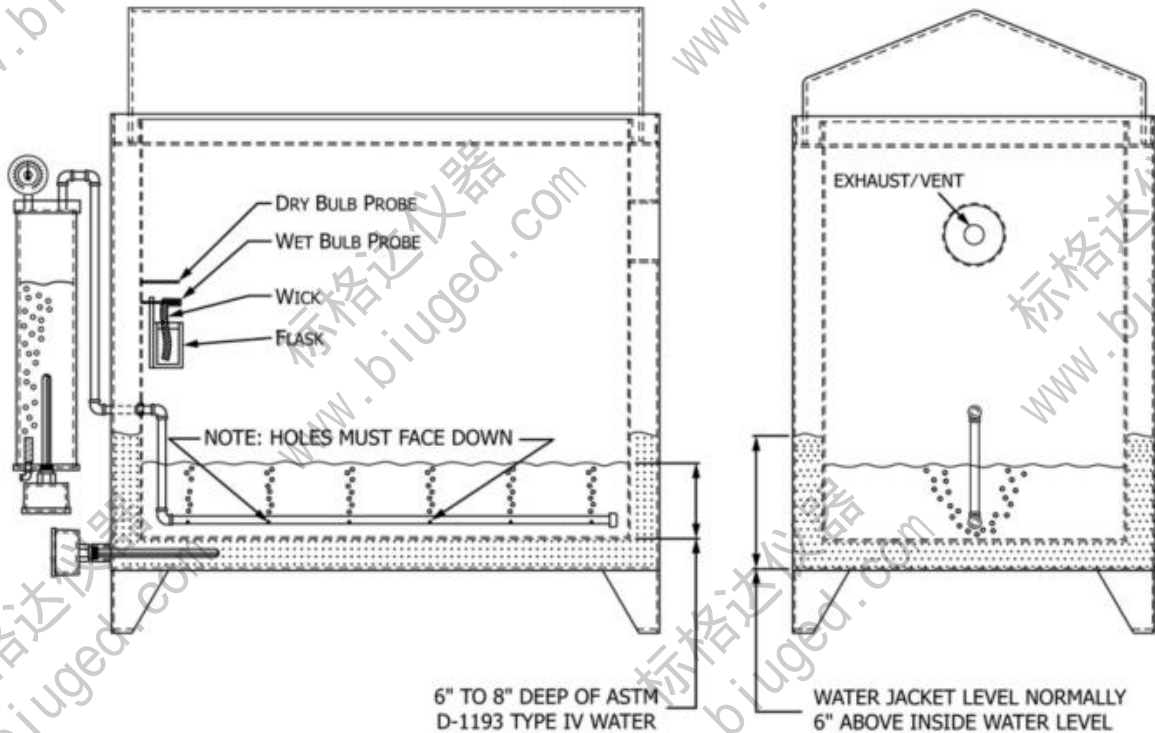
FIG. X1.3 Cyclic Corrosion Tester Cabinet with Vapor Generator
