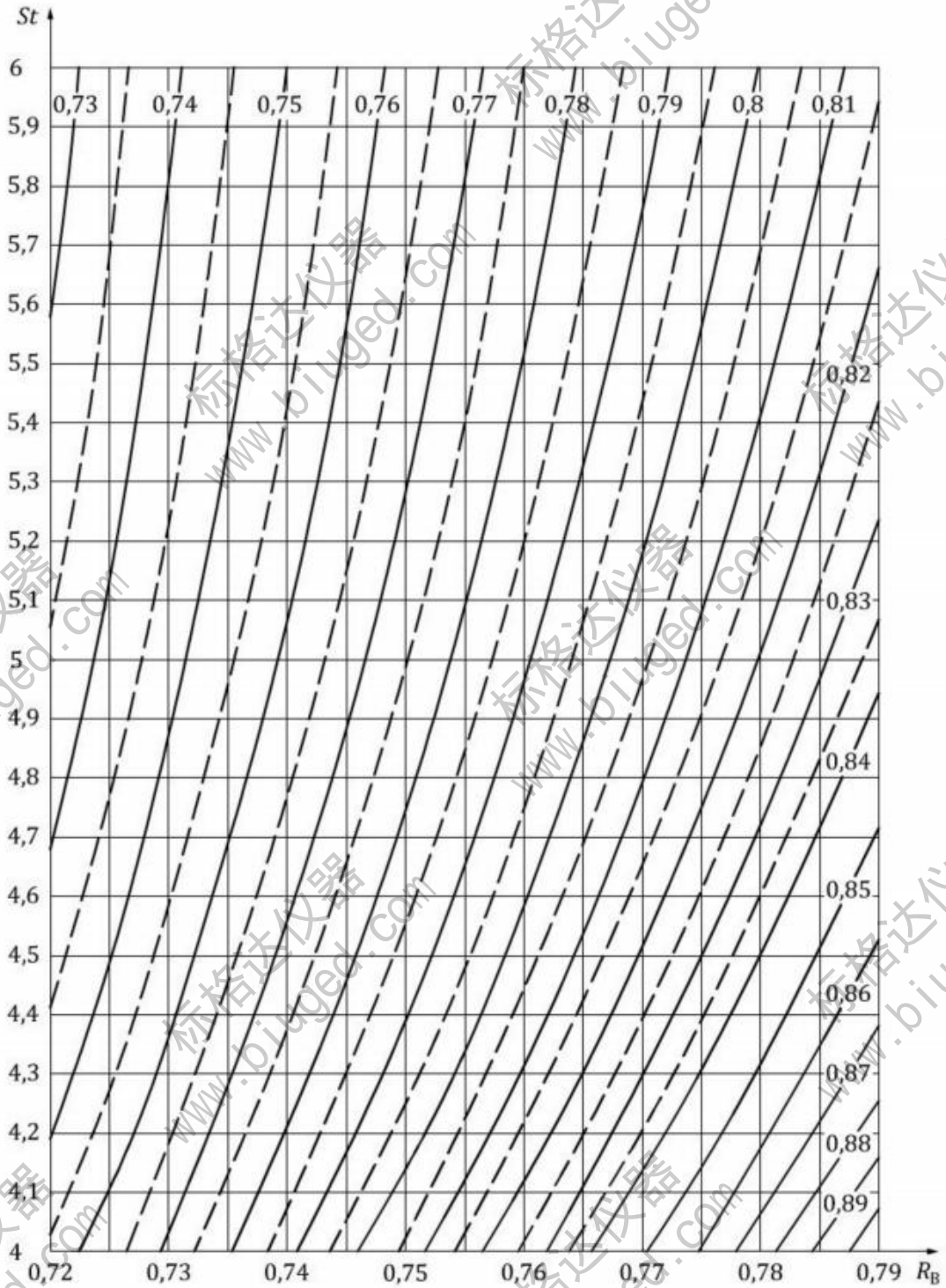
Figure A.9 — Values of St for the ranges 0,72 \leq R_B \leq 0,79 0,73 \leq R_\infty \leq 0,89
