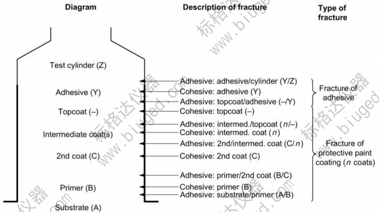
Figure 1 — Description of types of fracture
